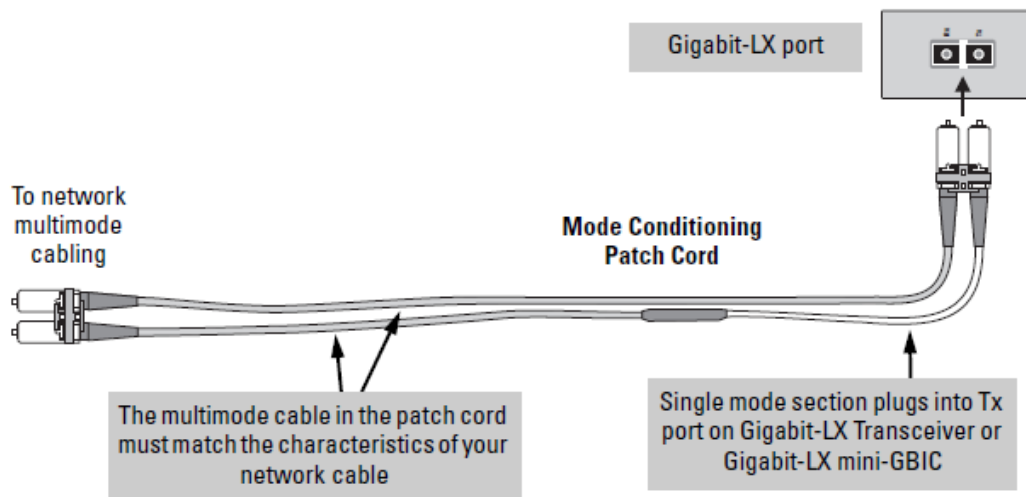
Figure 1 Example: Connecting a Mode Conditioning Patch Cord for Gigabit-LX
